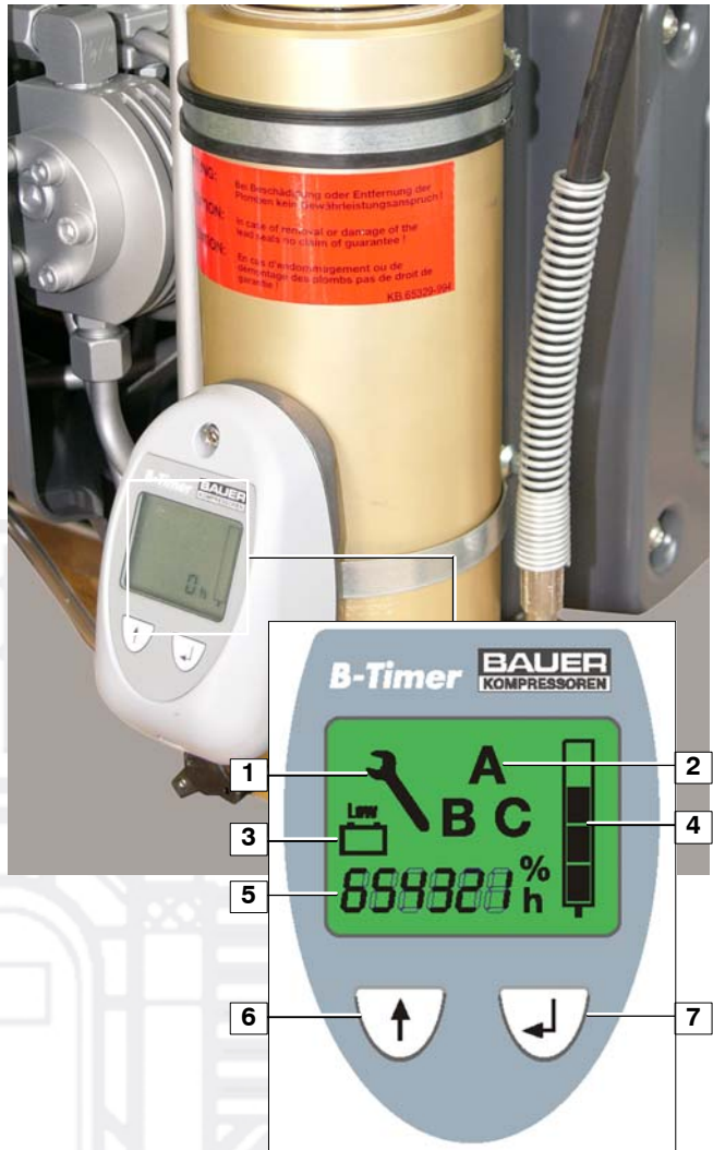
Abb. 13 B-Timer
